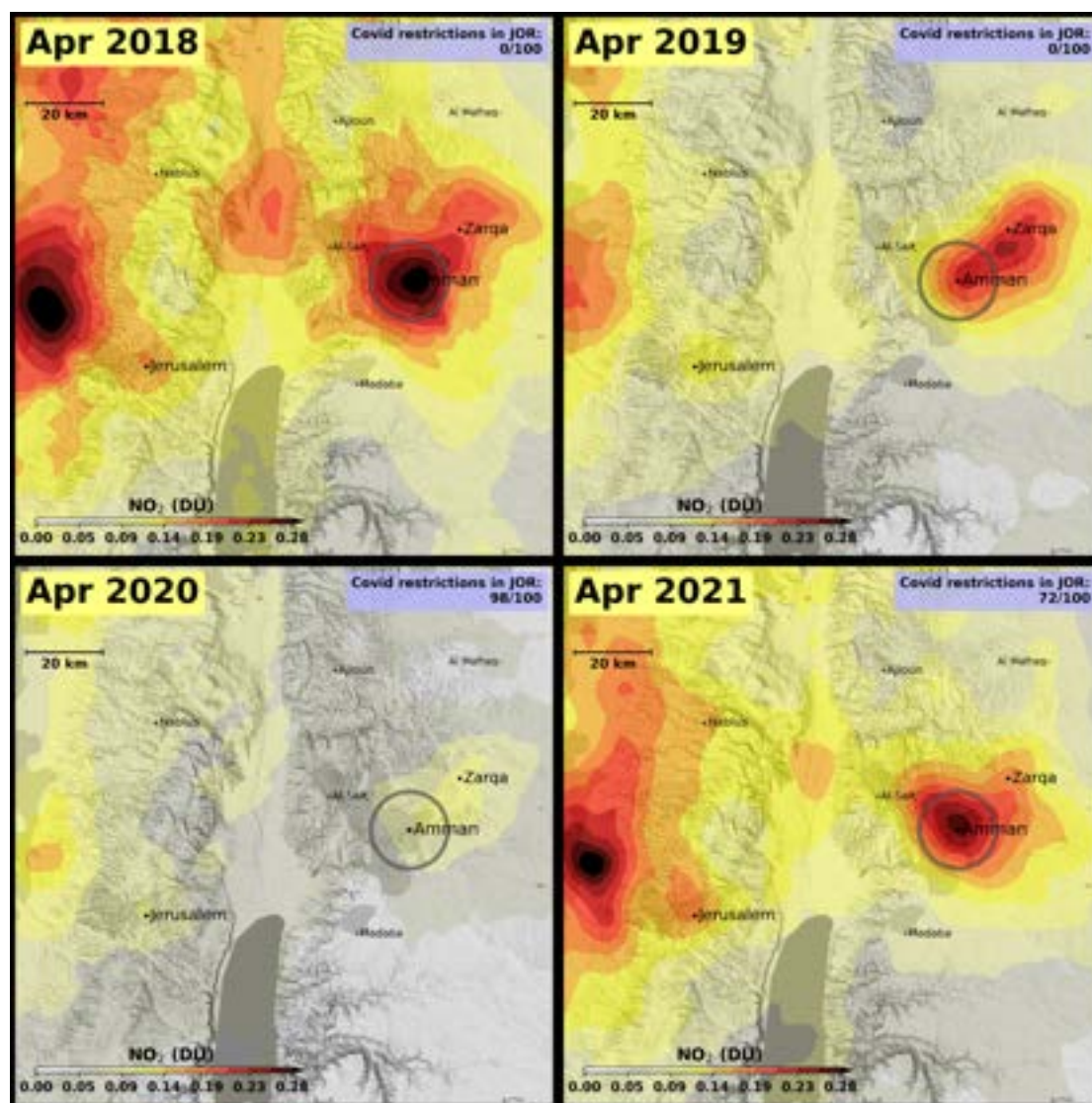
Maps: NO 2 column amount in April 2018 through 2021 in the Amman area. The circle has a 10km radius around the city centre.
