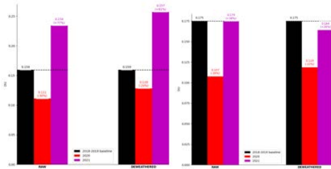
Left bar chart: April NO 2 column amount in Gauteng (left bars: raw data, right bars: deweathered data). Right bar chart: Same for Mpumalanga.
