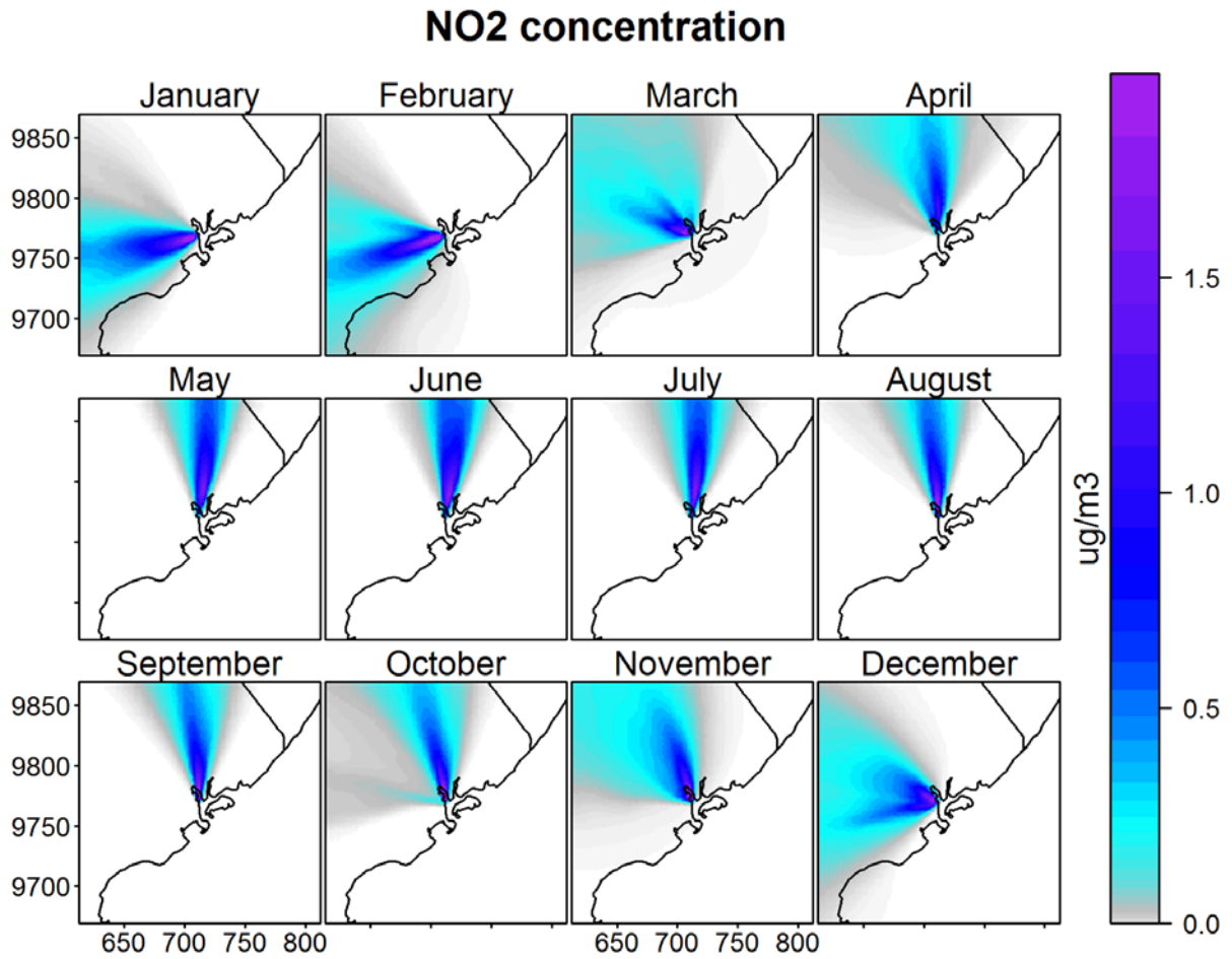
Figure 5 Projected monthly average NO 2 concentrations caused by emissions from the Lamu power plant ( \mu\text{g}/\text{m}^3 )
