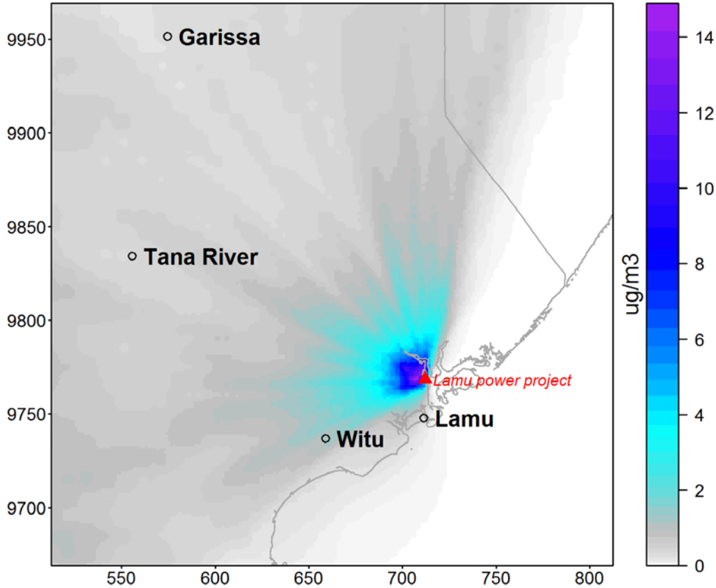
Figure 7 Projected 24-hour maximum SO 2 concentrations caused by emissions from the Lamu power plant (µg/m 3 )
