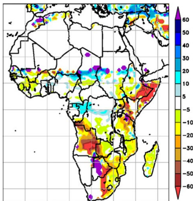
Figure 2. Percentage change in growing season days (GSDs) for 2041-2060 predicted using a regional climate model at a 90 km resolution. Expressed as a percent change from the number of days in the mean value at each grid point. Based on Cook & Vizzy (2012).
